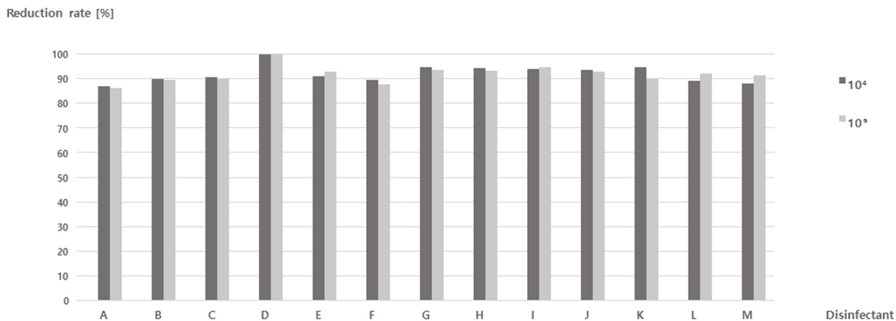
Figure 1. Reduction effect of 13 disinfectants in bacterial suspension experiment
