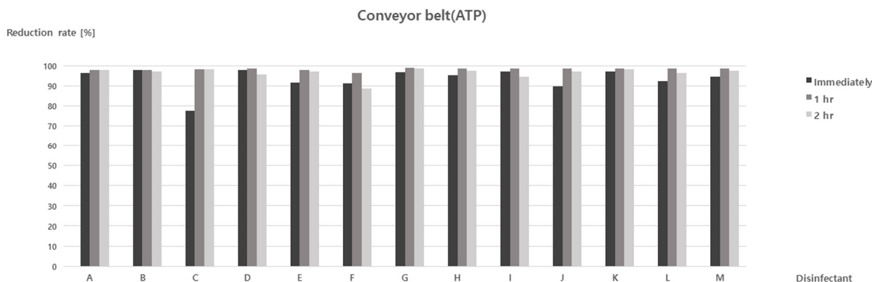
Figure 9. Bacterial reduction rate of 13 disinfectants in conveyor by ATP measuring instrument
